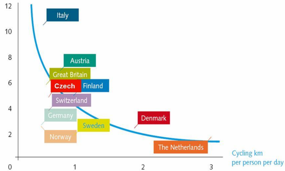
Killed cyclists per 100 million km
